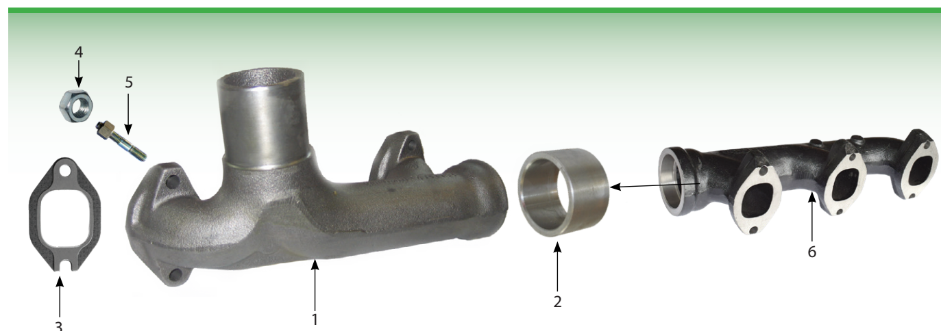
1. 7364 Exhaust Manifold Fiat 100-90 100-90DT 2. 7365 Exhaust Manifold Coupling Fiat 100-90 3. 7360 Exhaust Manifold Gasket All Models Pack of 6 4. 3002 Nut M8 Metric Coarse Zinc & Yellow 5. 7590 Exhaust Manifold Stud Fiat 6. 7366 Exhaust Manifold Fiat 100-90 100-90DT
