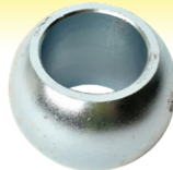
Lower Link Ball Cat 3/2 ID 29 OD 63.5
