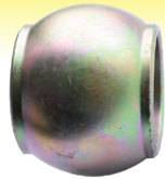
Lower Link Ball 57mm OD 36.5mm ID 44.5 Width
