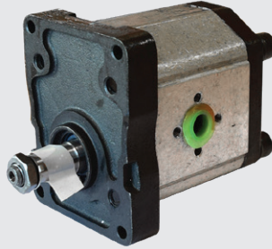
7761 Hydraulic Pump 42 Ltr Fiat 70 - 110 OE Ref: 5129488 84530156
